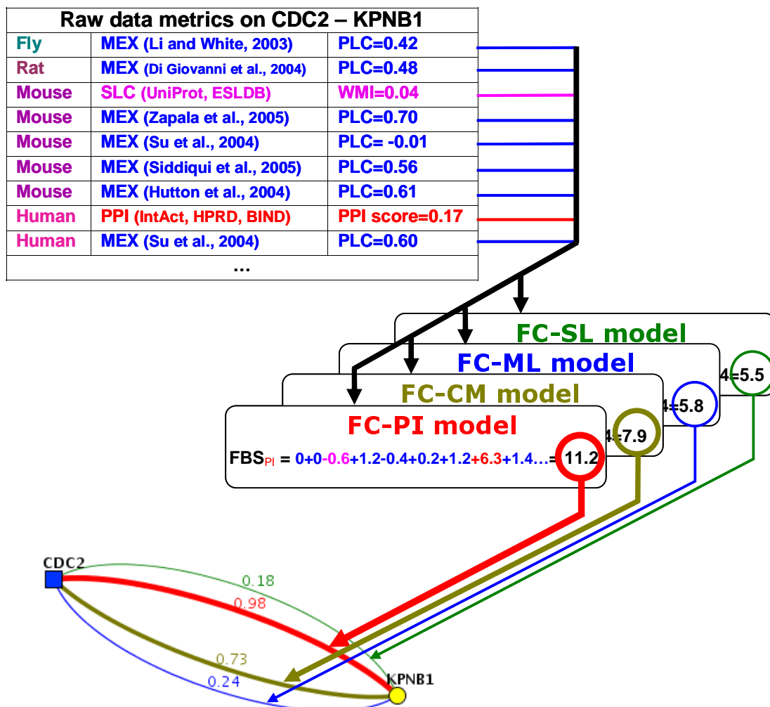
Figure 2. Example of predicting functional coupling by FunCoup's Naïve Bayesian Network. To evaluate the cumulative likelihood of the link CDC2 – KPNB1 , several (only 9 shown) evidences from a number of species were available. The metrics computed from each evidence were scored by the 4 models of functional coupling and summed up to a total likelihood value, the Final Bayesian Score (FBS). In this example, a physical protein interaction (FC-PI) is more likely than membership in the same protein complex (FC-CM), a metabolic (FC-ML), or a signaling (FC-SL) link. The web interface to the database of predictions ( http://FunCoup.sbc.su.se ) displays likelihoods of the FC classes as 4 coloured lines with FBS values transformed into the pfc confidence scores.
