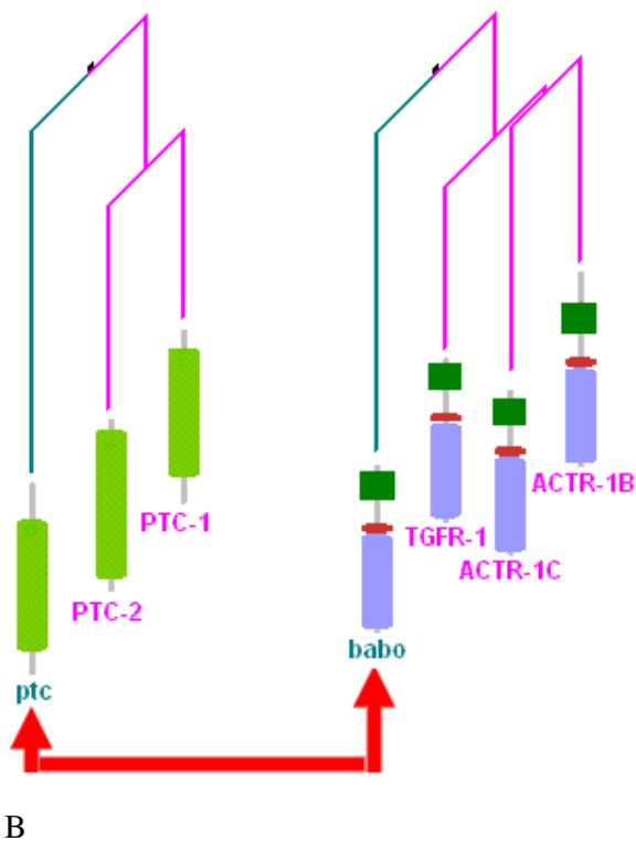
Figure 4. Scenarios for interaction inheritance.
