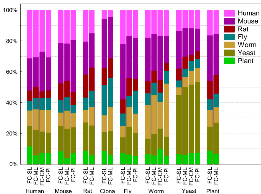
Figure 3. Relative evidence contribution to FunCoup networks viewed by input data type (A) or species (B). For each evidence category in each species and FC class, we calculated the sum of its contributions to the final Bayesian score (FBS) over the whole predicted network, i.e. the set of links with FBS > 3 . Then, these sums were normalized by dividing with the sum of FBS scores over the same set. Note that no input data from Ciona was used. Data type legends as in Figure 1.
